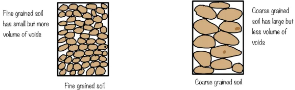
Fig:2 Comparison of void ratio
